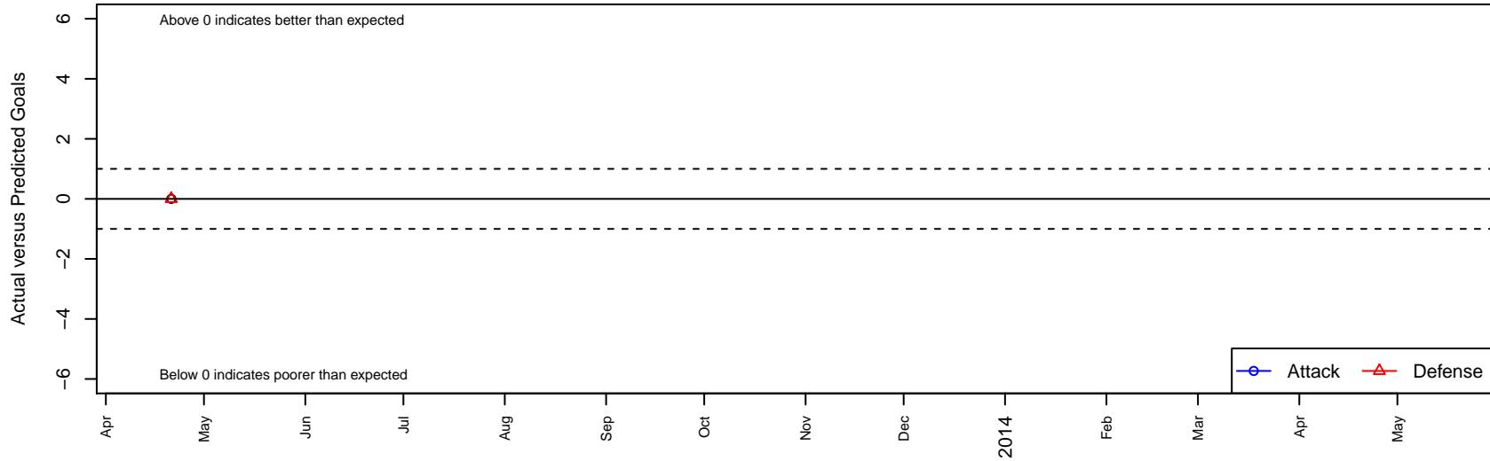
NEU Internazionale B99 Dots are actual minus expected GF (blue circles) and GA (red triangles). Blue line is smoothed change in attack strength. Red is smoothed change in defense strength.
